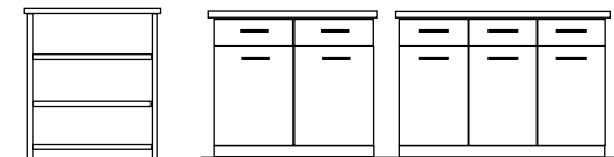
Small Bookcase H 920 W 780 D 320
